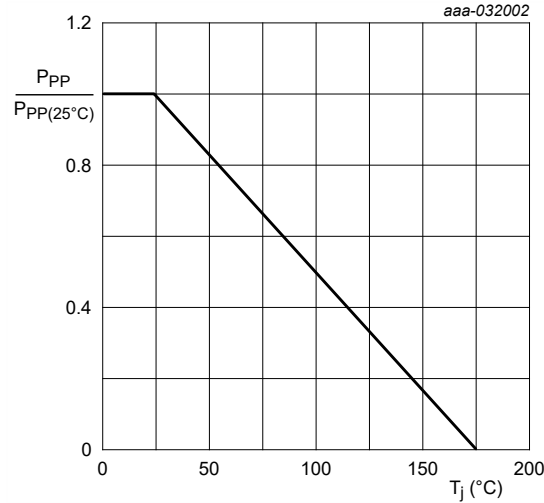
Fig. 7. Relative variation of peak pulse power as a function of junction temperature; typical values
